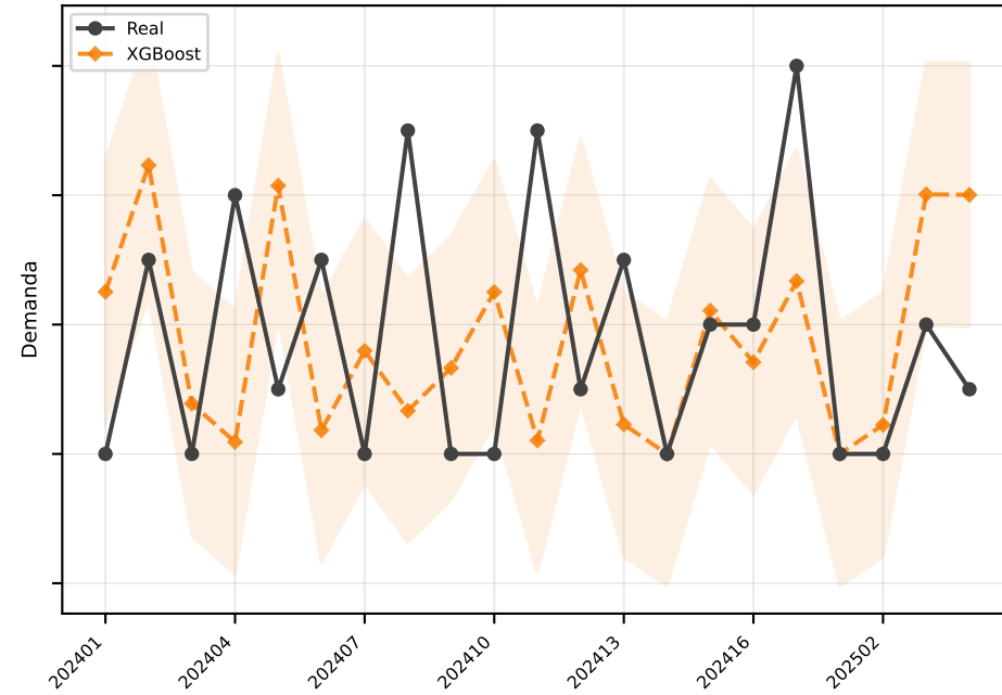
XGBoost MAE=2.0
