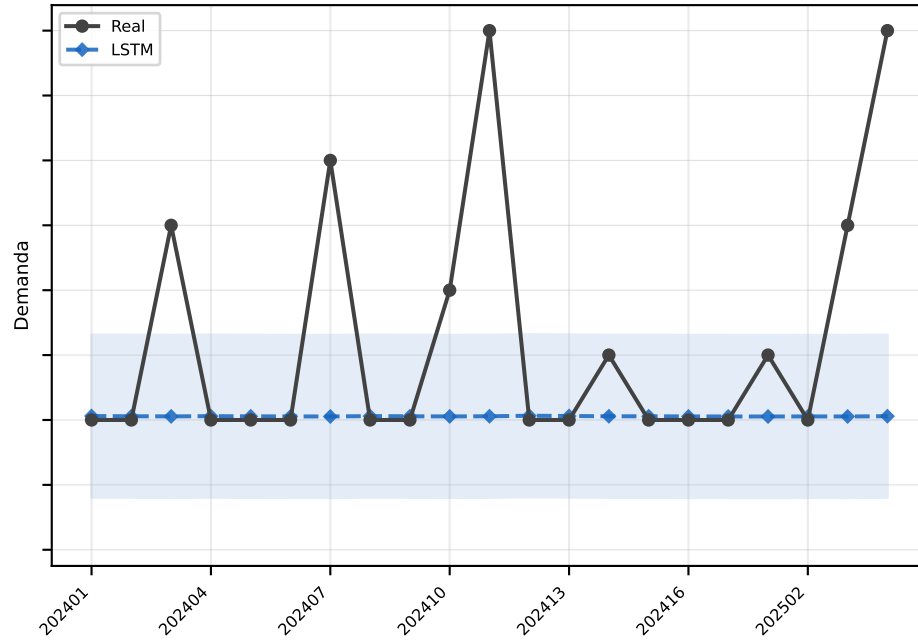
LSTM MAE=1.3
