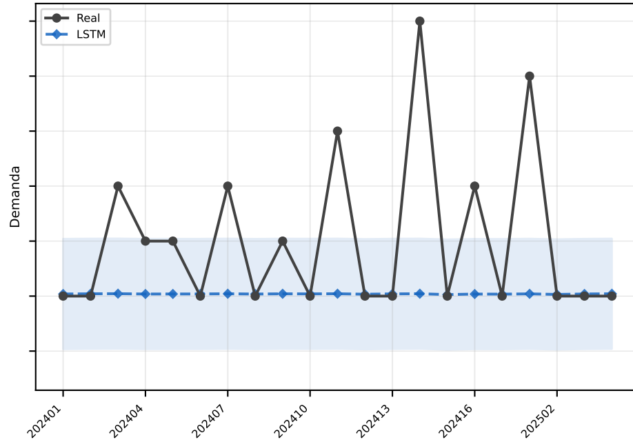
LSTM MAE=1.0
