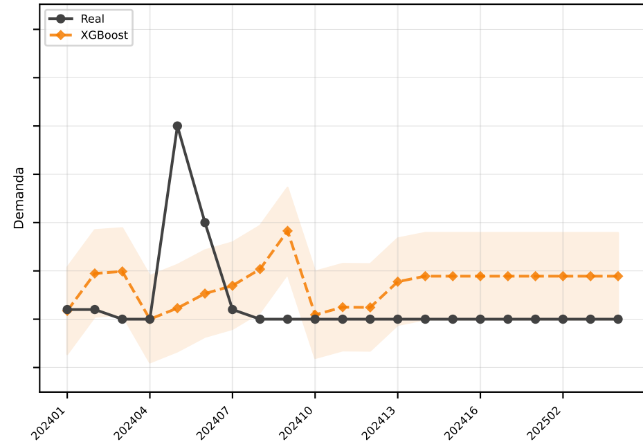
XGBoost MAE=4.5
