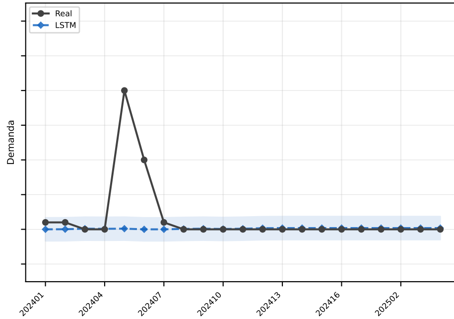
LSTM MAE=1.7
