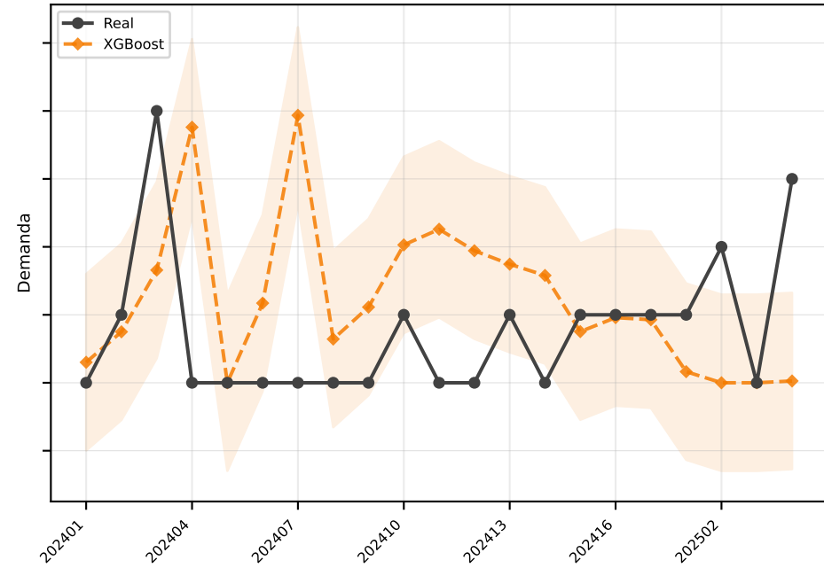
XGBoost MAE=1.3
