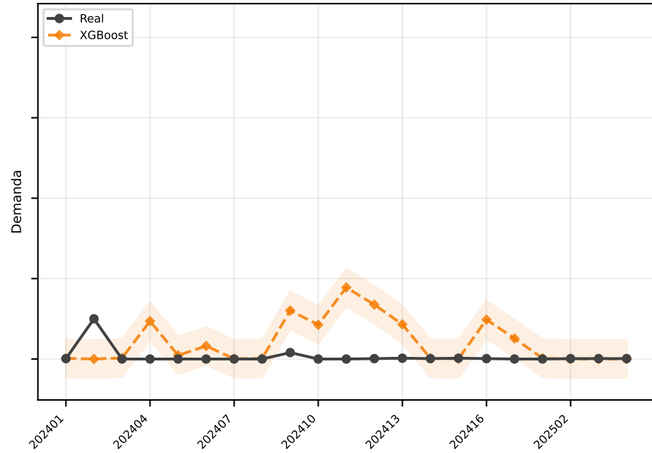
XGBoost MAE=46.8
