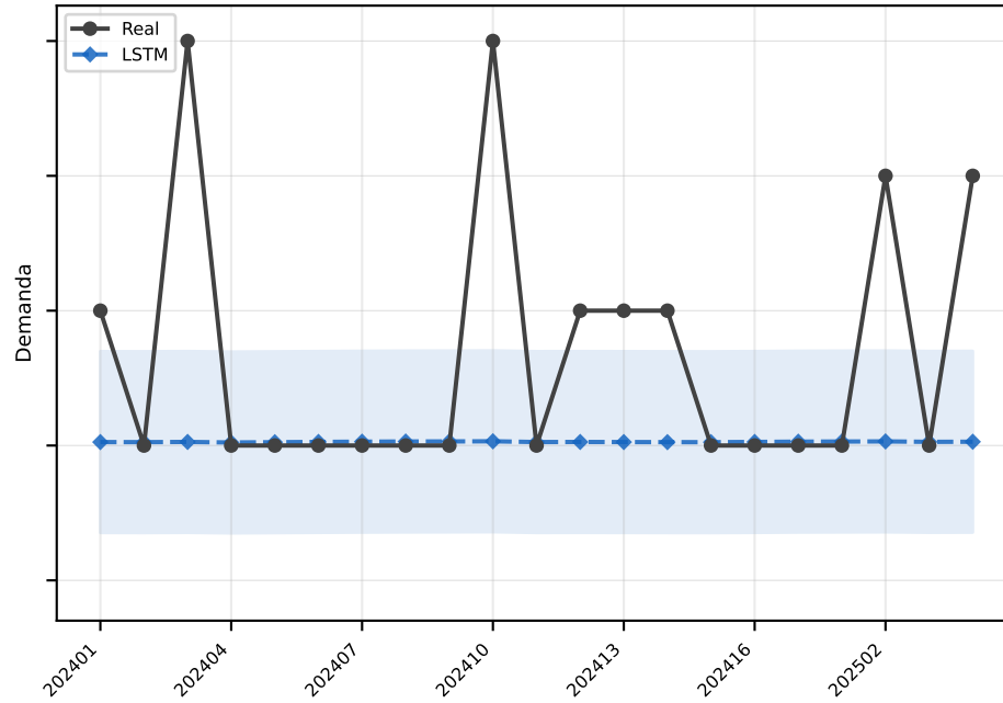
LSTM MAE=0.7
