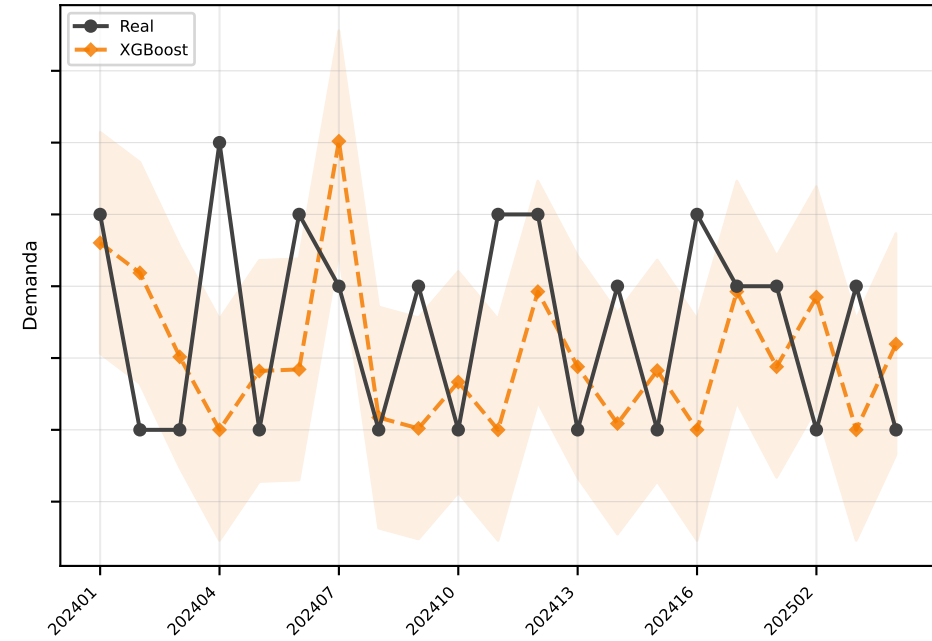
XGBoost MAE=1.5
