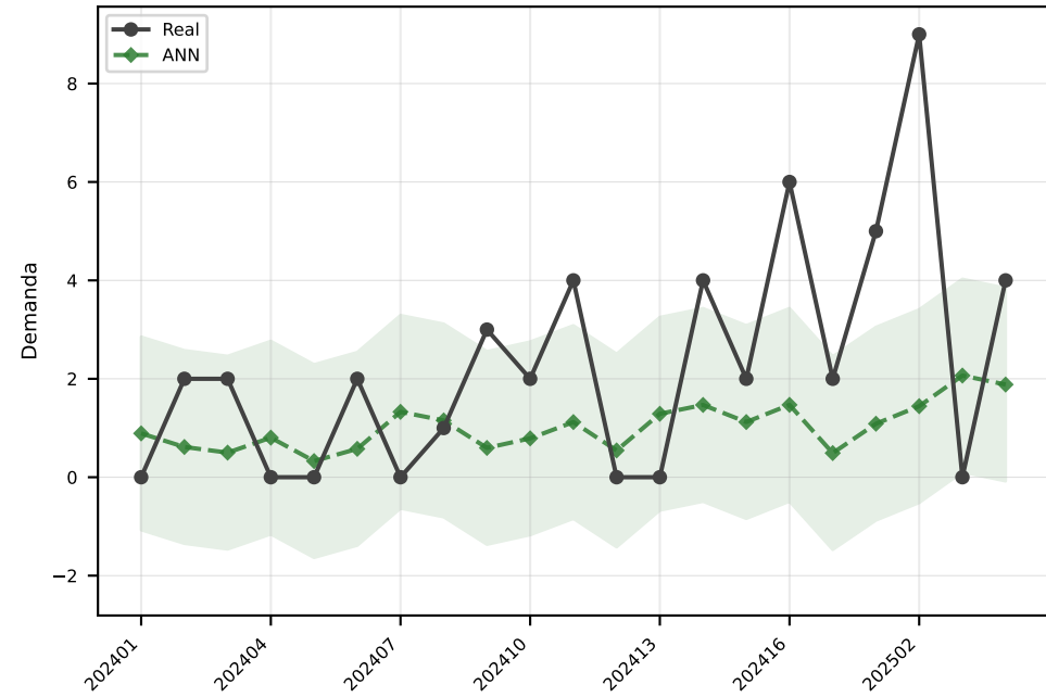
ANN MAE=2.0
