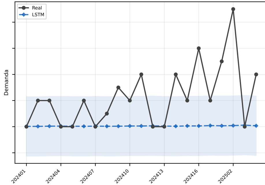
LSTM MAE=2.3
