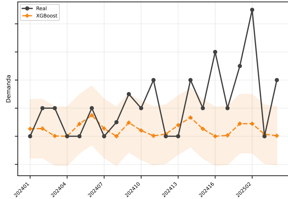
XGBoost MAE=2.1
