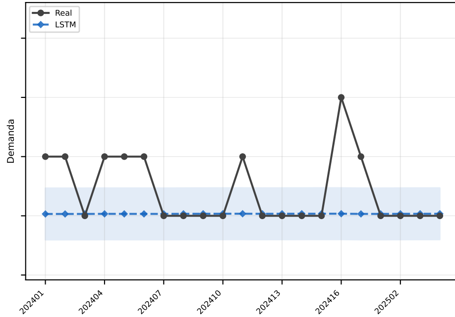
LSTM MAE=0.4
