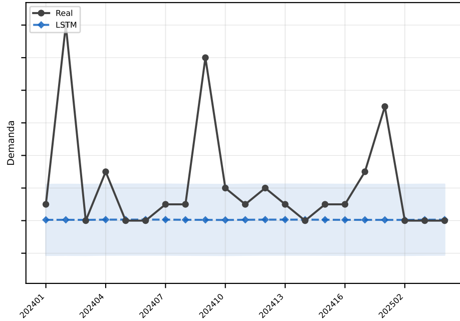
LSTM MAE=2.2
