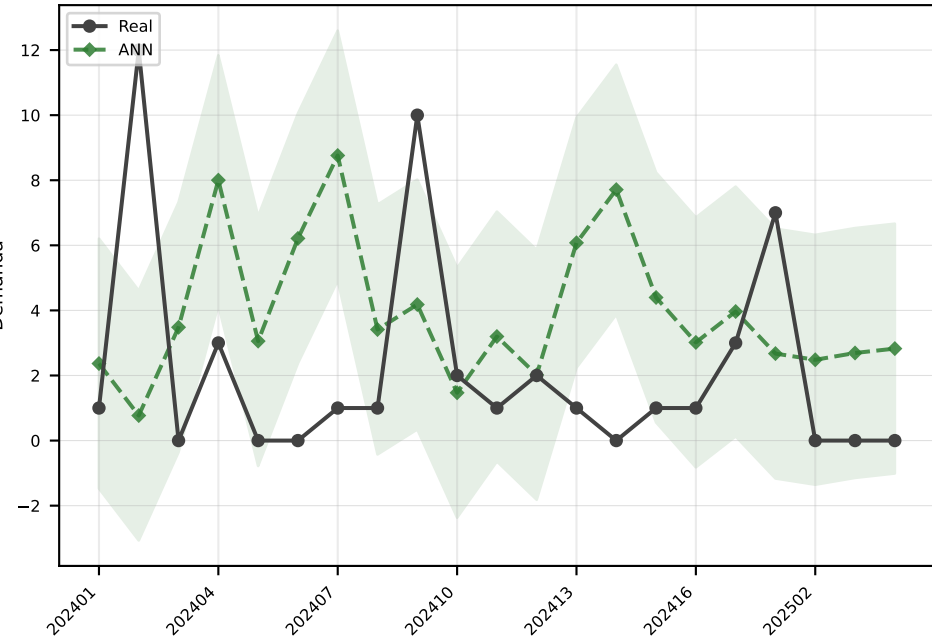
ANN MAE=3.8
