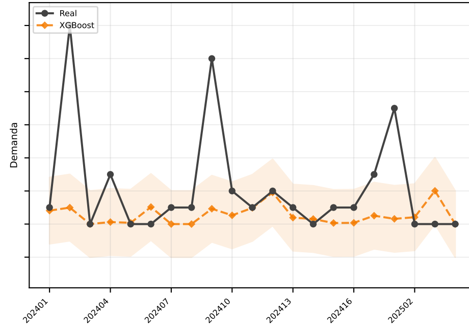
XGBoost MAE=2.0
