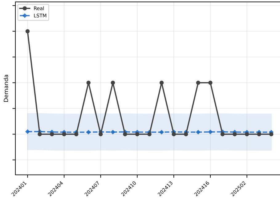
LSTM MAE=0.4
