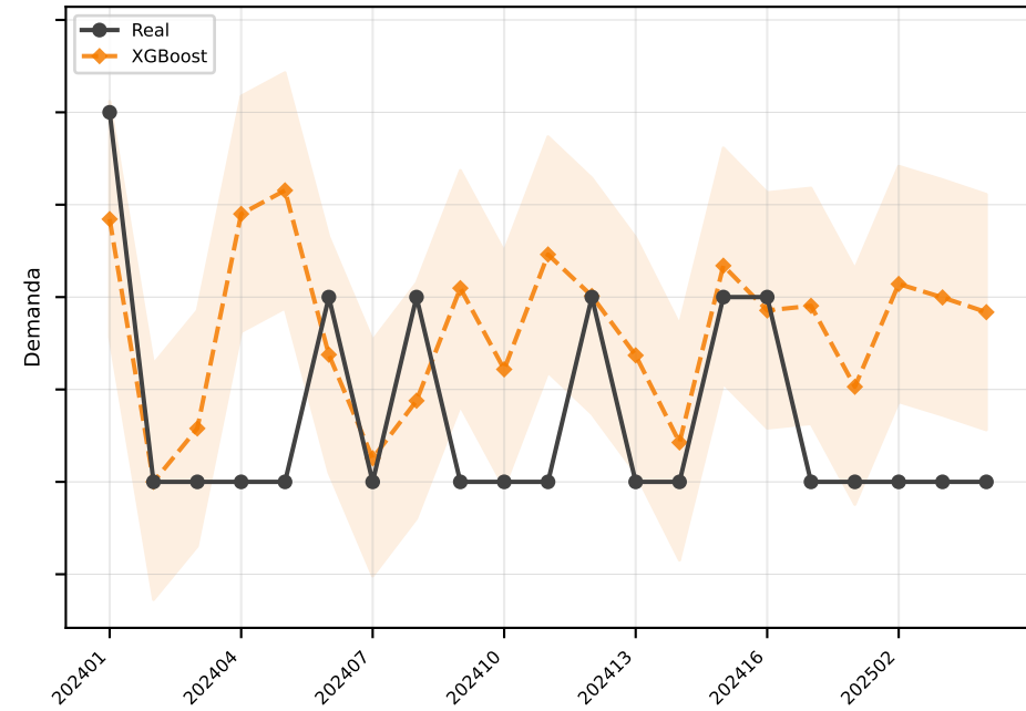
XGBoost MAE=0.6
