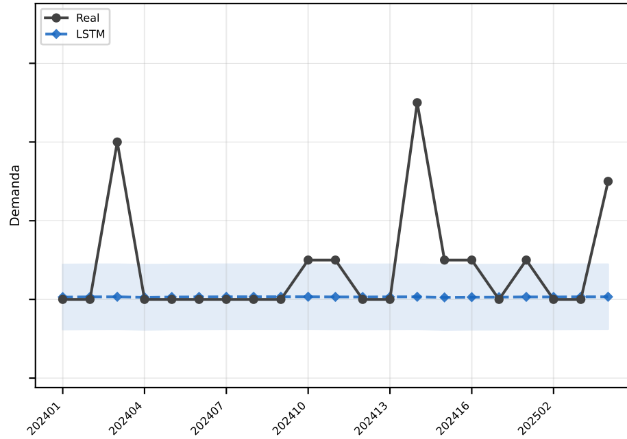
LSTM MAE=0.8
