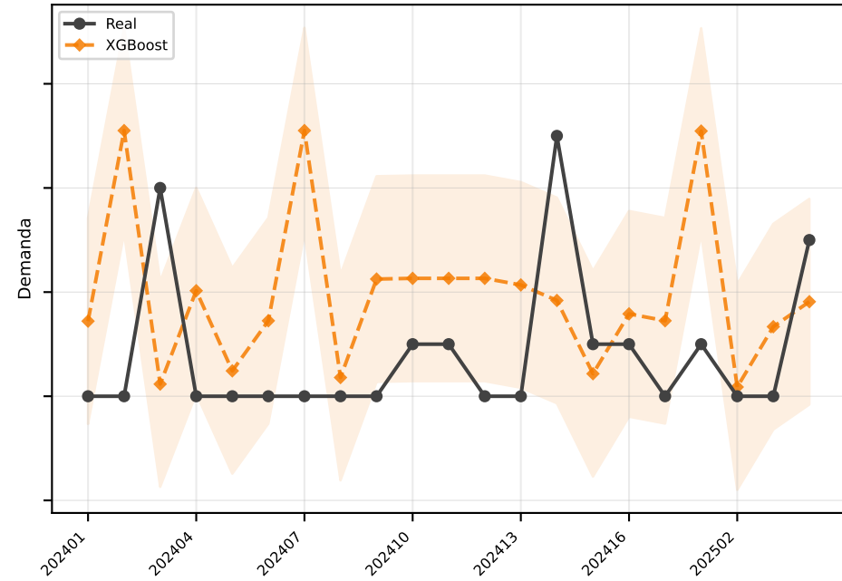
XGBoost MAE=2.0
