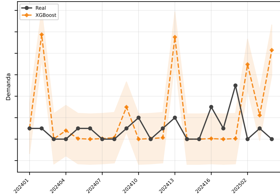
XGBoost MAE=2.4
