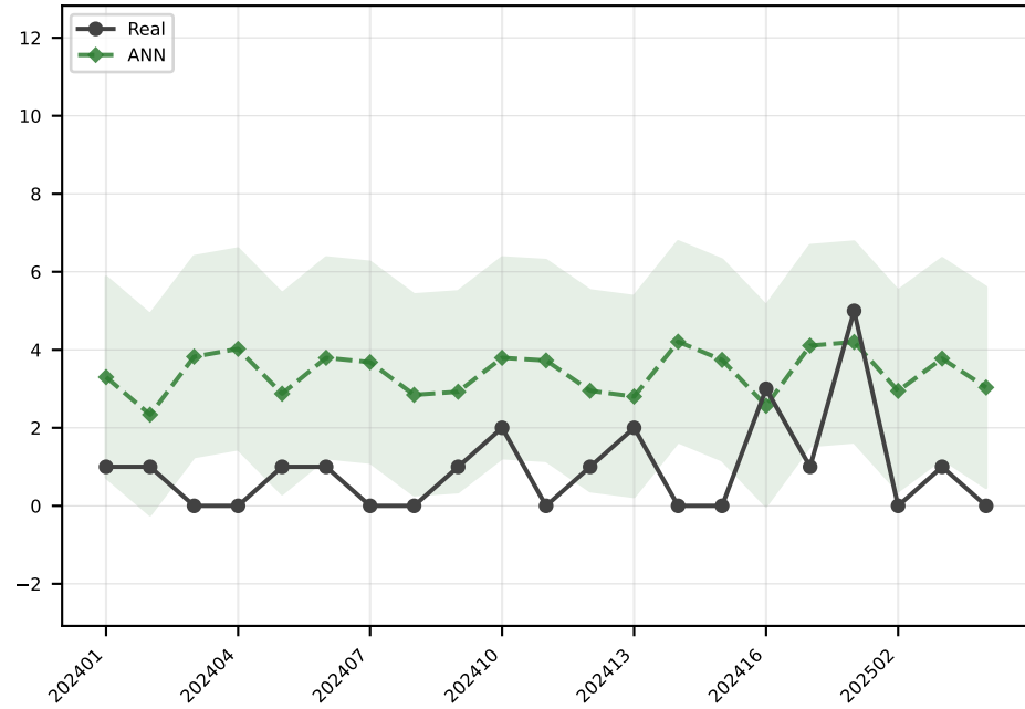
ANN MAE=2.6
