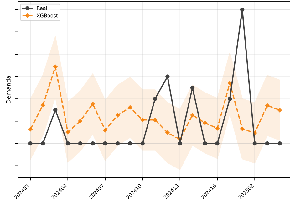
XGBoost MAE=2.7
