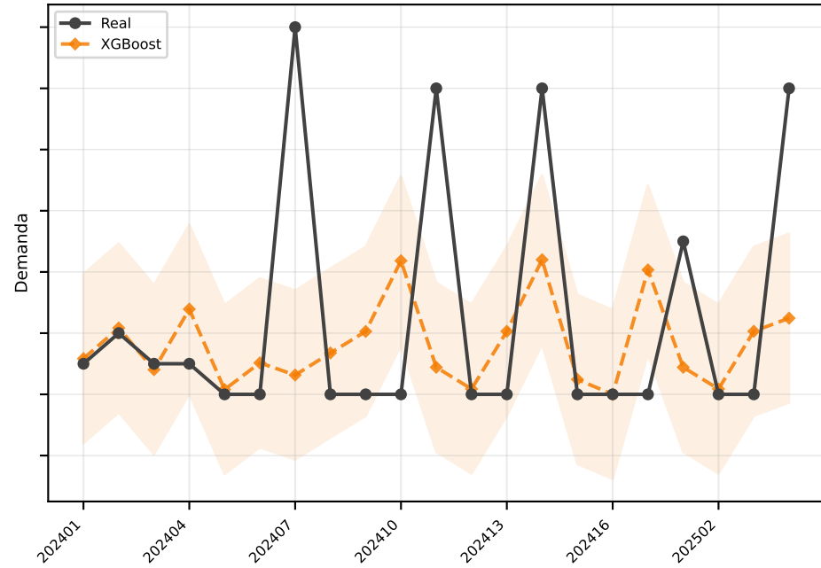
XGBoost MAE=2.8
