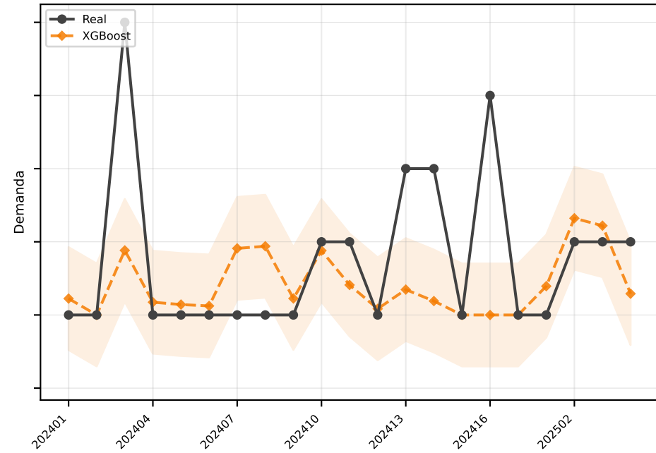
XGBoost MAE=0.7
