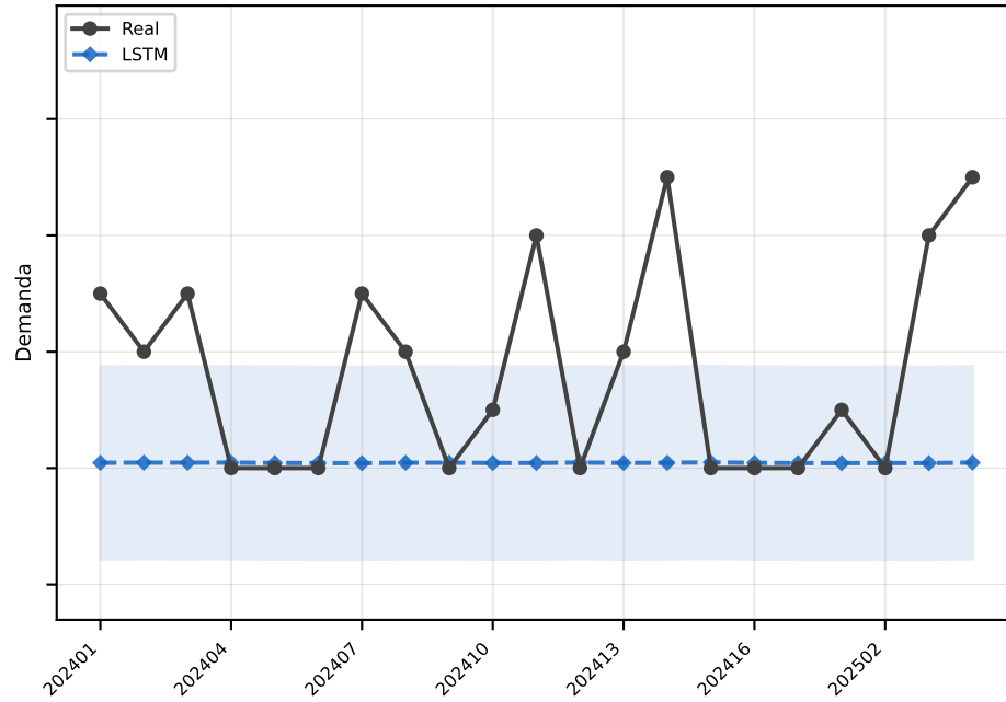
LSTM MAE=1.7
