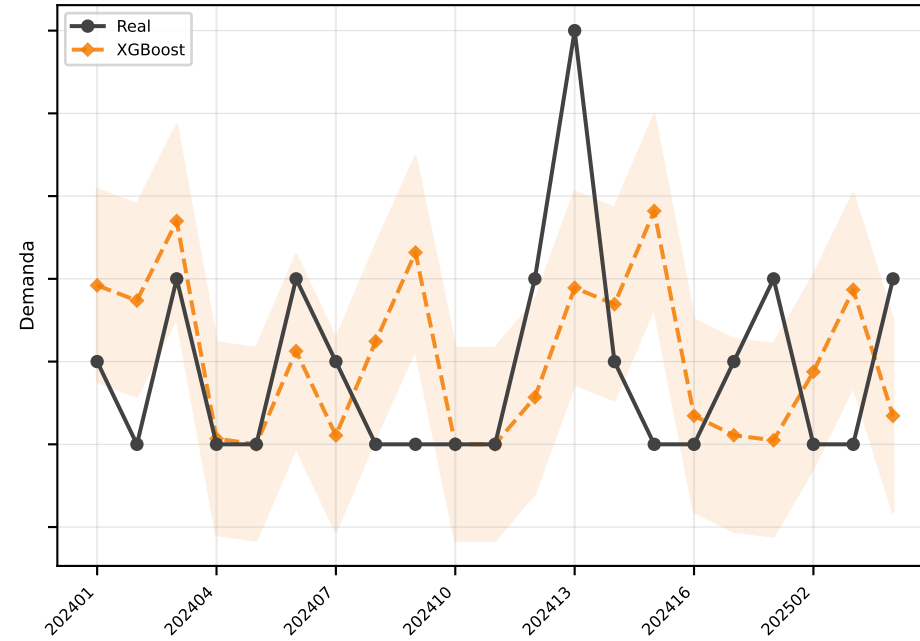
XGBoost MAE=1.2
