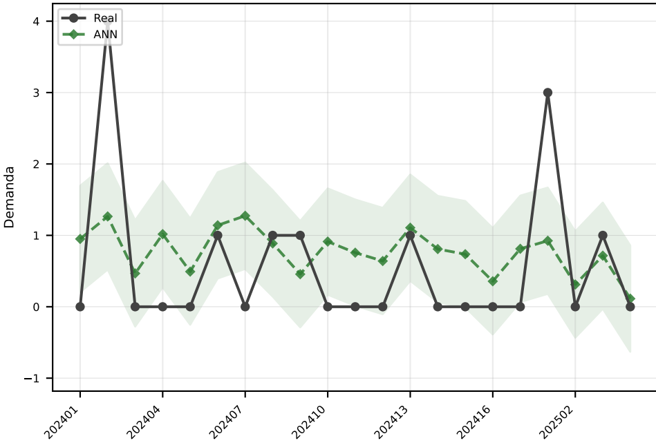
ANN MAE=0.7
