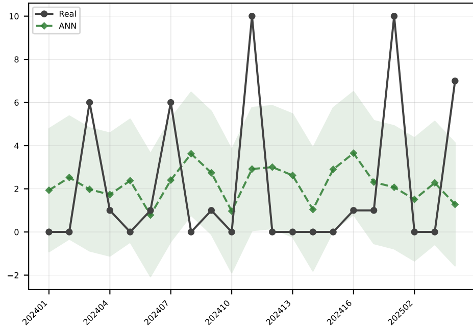
ANN MAE=2.8
