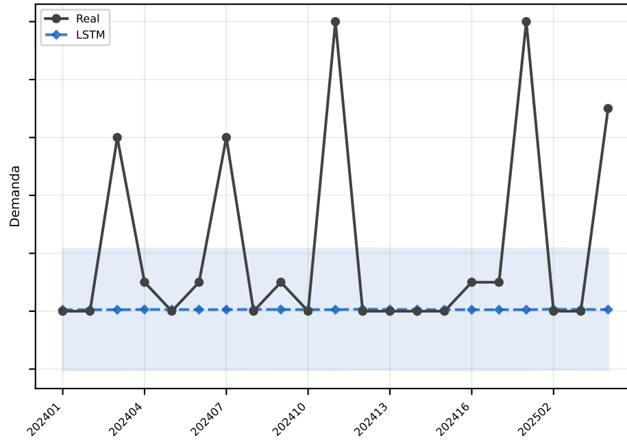
LSTM MAE=2.1
