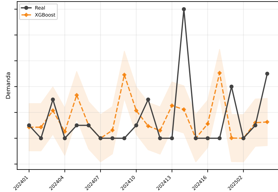
XGBoost MAE=1.8
