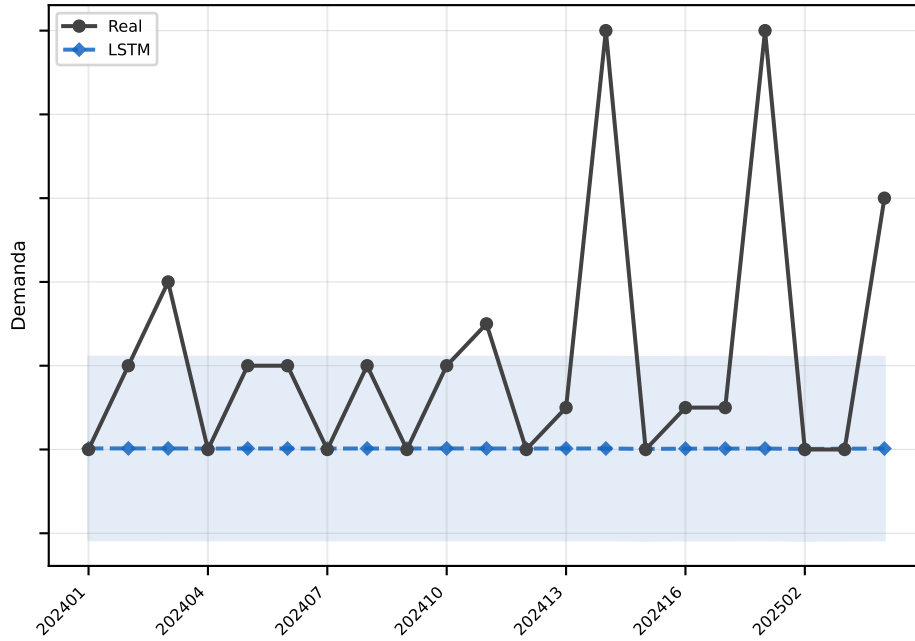
LSTM MAE=2.2
