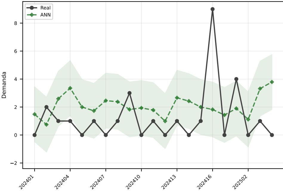
ANN MAE=2.0
