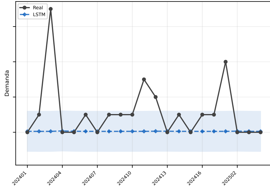
LSTM MAE=1.1
