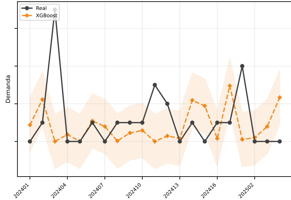
XGBoost MAE=1.4
