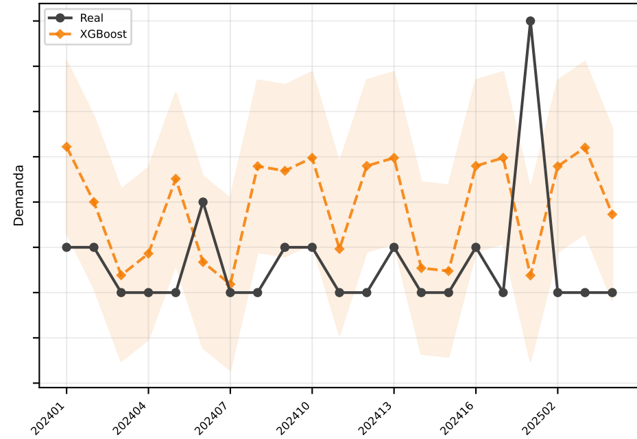
XGBoost MAE=1.9
