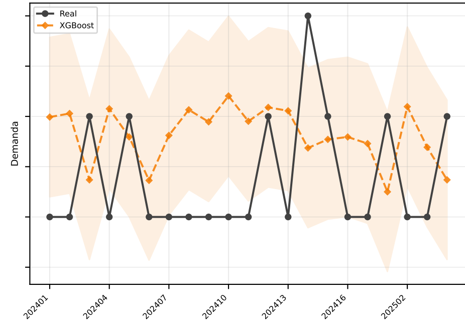
XGBoost MAE=0.8
