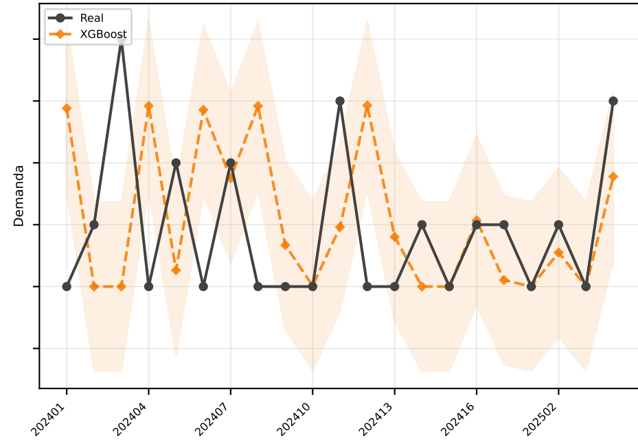
XGBoost MAE=1.4
