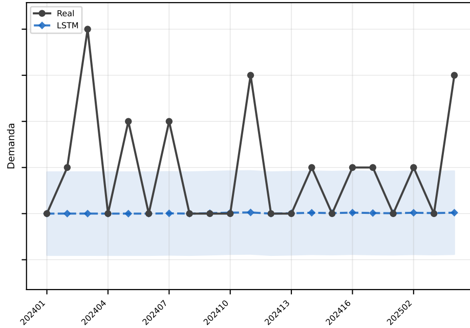
LSTM MAE=0.9
