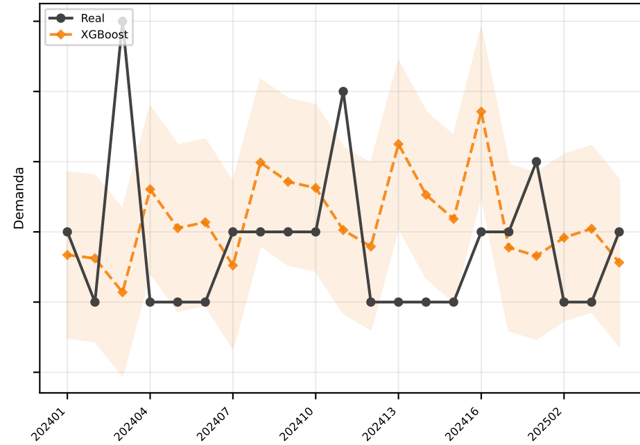
XGBoost MAE=1.2
