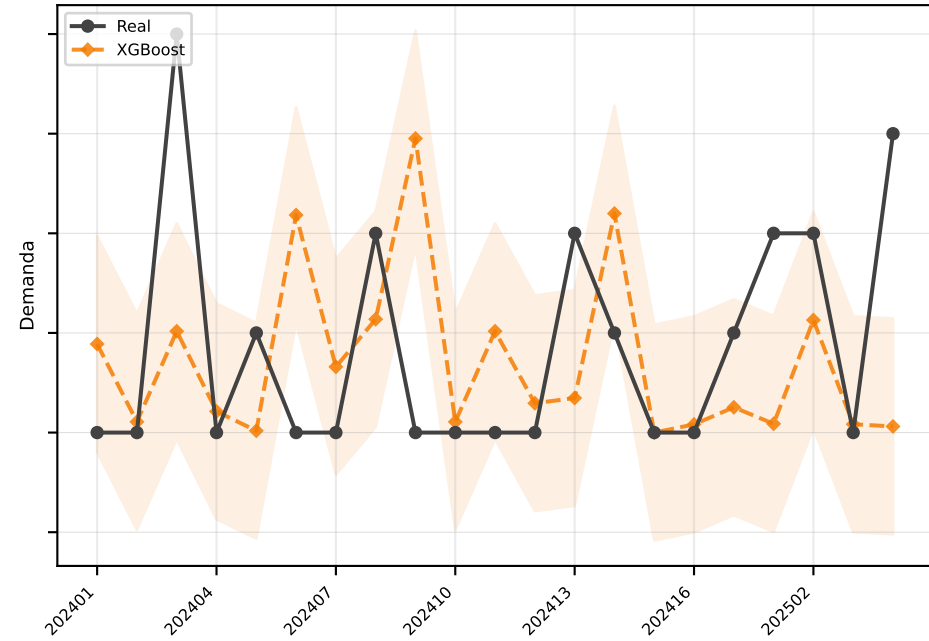
XGBoost MAE=1.1
