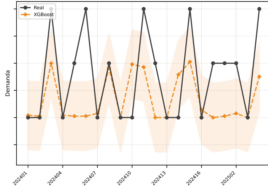
XGBoost MAE=0.6
