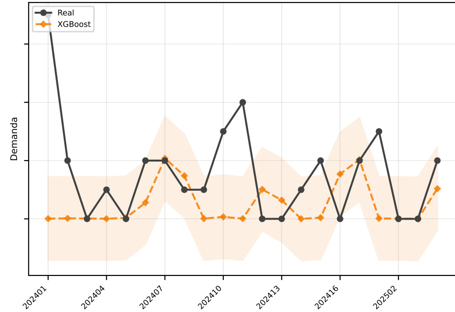
XGBoost MAE=1.4
