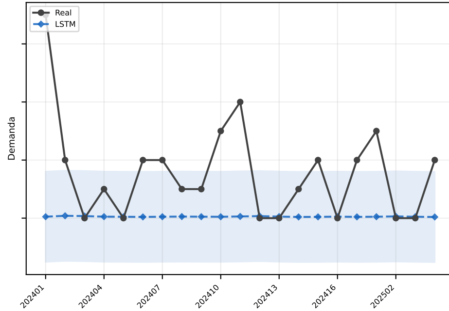
LSTM MAE=1.6
