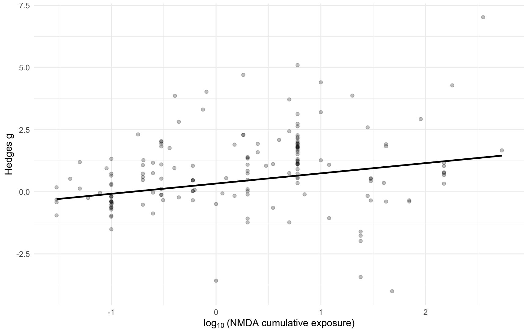
Meta-regression: log cumulative exposure vs effect size (Rat+Mouse)
