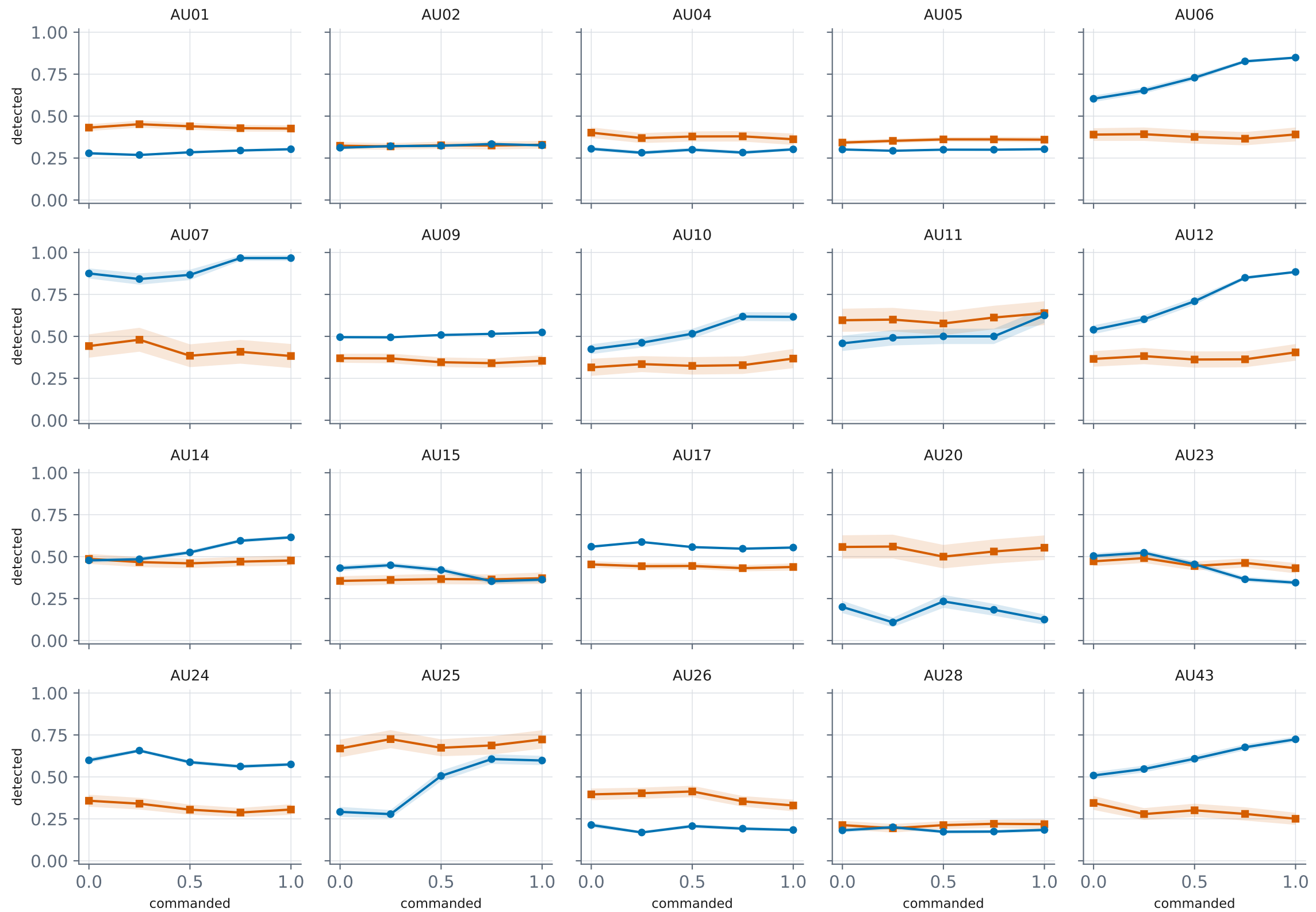
AU co-activation trajectories: detected presence vs commanded AU12 (blue=trained, orange=baseline)
