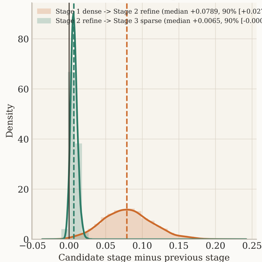
Bootstrap delta: Spearman
