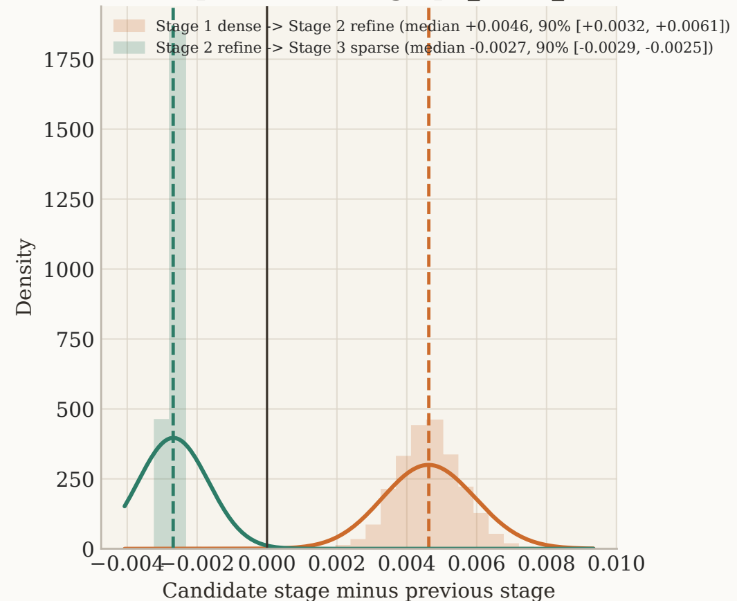
Bootstrap delta: mean graph_score_mean
