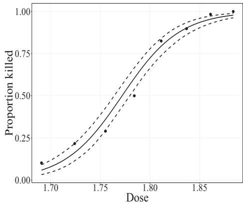
Figure 14.2 Observed proportion killed (dots), estimated logit dose response model (solid line) and 95% posterior intervals (dotted lines) from a Bayesian model for the beetle mortality data from Table 7.2 .
