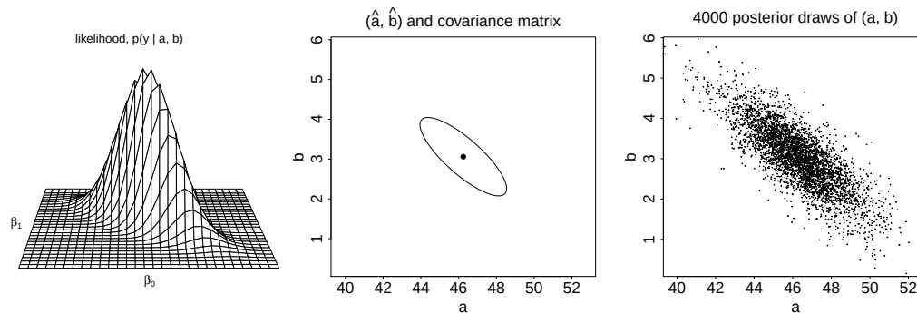
Figure 9.4 (a) Reproduced from Figure 8.1a: Likelihood function for the parameters a and b in the linear regression y = a + bx + \text{error} , of election outcomes, y_i , on economic growth, x_i . (b) Reproduced from Figure 8.1c: Mode of the likelihood function with an ellipse summarizing the inverse-second-derivative-matrix of the log likelihood at the mode. (c) 4000 random simulation draws (a, b) from the posterior distribution corresponding to a flat prior.
