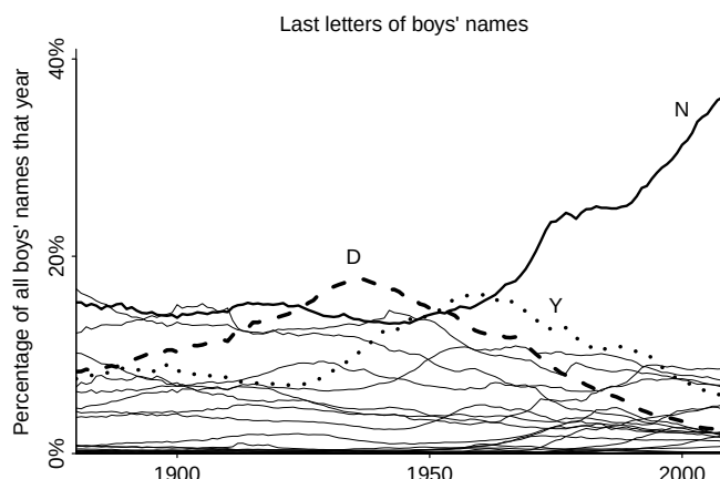
Figure 2.8 Trends in percentage of boys' names ending in each letter. This graph has 26 lines, with the lines for N , D , and Y in bold to show the different trends in different-sounding names. Compare to Figures 2.6 and 2.7, which show snapshots of the last-letter distribution in 1906, 1956, and 2006.
