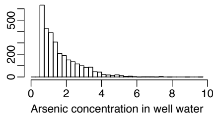
Figure 13.9 Histogram of arsenic levels in unsafe wells (those exceeding 0.5) in the measured area of Araihaaz, Bangladesh (see Figure 13.7).
