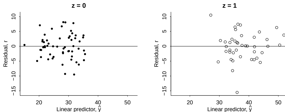
Figure 11.5 Continuing Figure 11.4, the residual, r = y - \hat{y} , vs. the fitted linear predictor \hat{y} , plotted separately for control and treatment groups.
