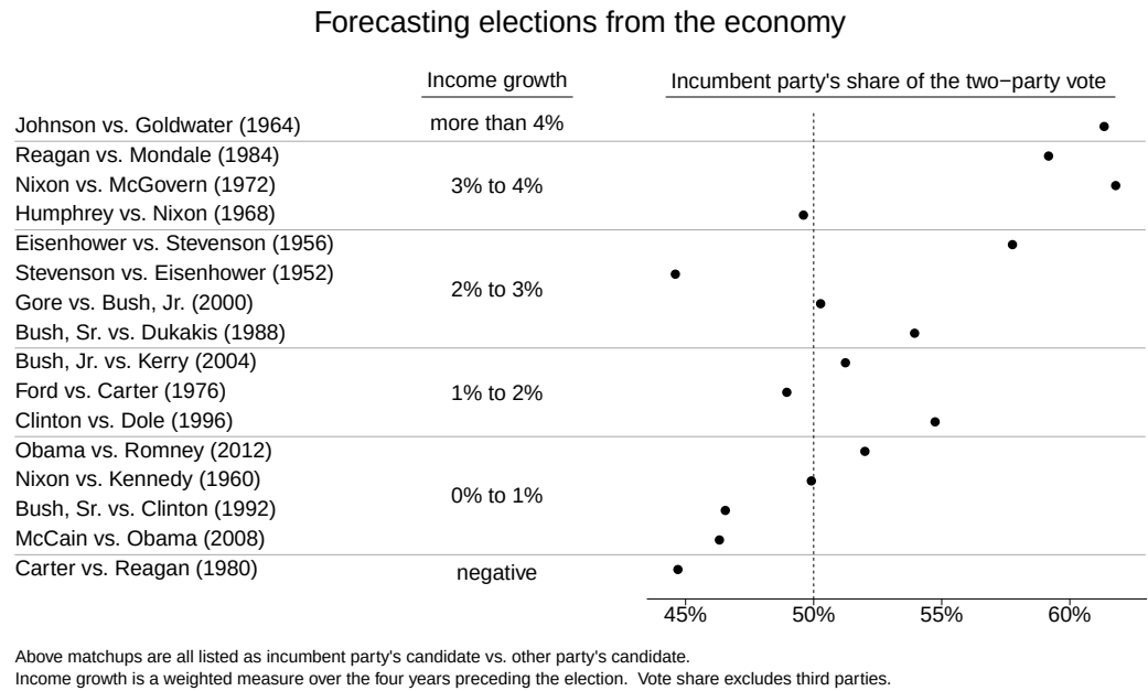
Figure 7.1 Douglas Hibbs's “bread and peace” model of voting and the economy. Presidential elections since 1952 are listed in order of the economic performance at the end of the preceding administration (as measured by inflation-adjusted growth in average personal income). Matchups are listed as incumbent party's candidate versus other party's candidate. The better the economy was performing, the better the incumbent party's candidate did, with the biggest exceptions being 1952 (Korean War) and 1968 (Vietnam War).
