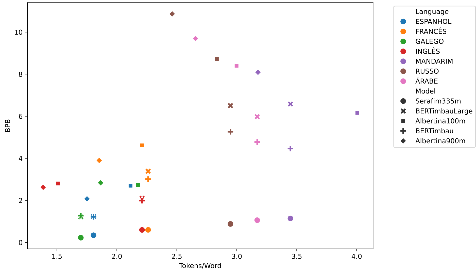
maskedLM - EXPLICAR
