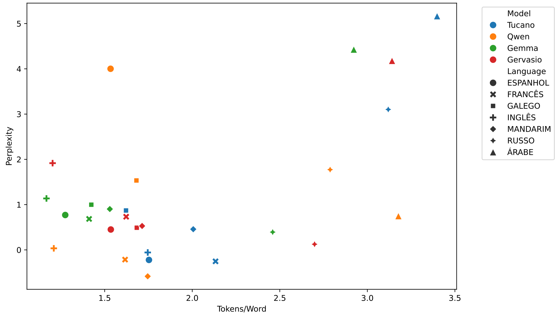
causalLM - RECOMENDAR
