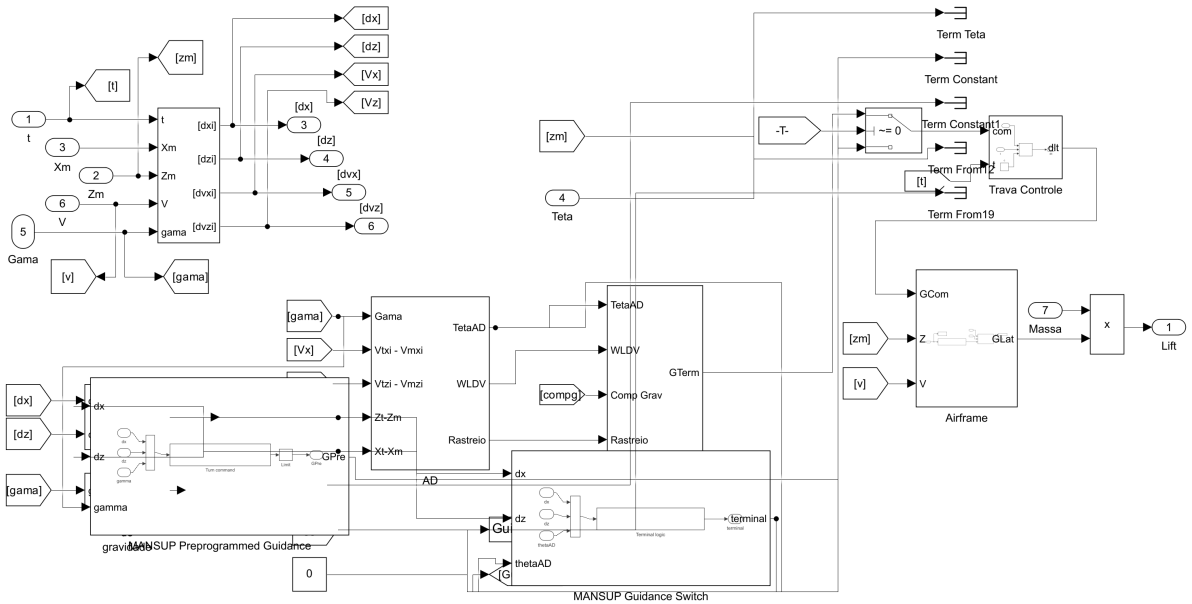
Figure 2: Modified control subsystem in the point-mass Simulink model.
