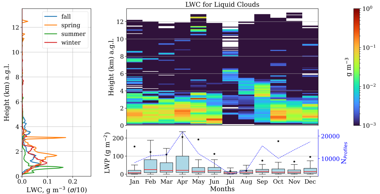
Figure 6. Seasonal average of liquid water content (LWC) and its monthly time series of LWC and liquid water path (LWP) for liquid clouds. Left panel shows the seasonal mean profiles of LWC, where shaded area indicates the standard deviation divided by 10. Right panel shows the monthly mean profiles of LWC and monthly box-plot of LWP. Boxplots are showing the median in red and the mean by black stars.
