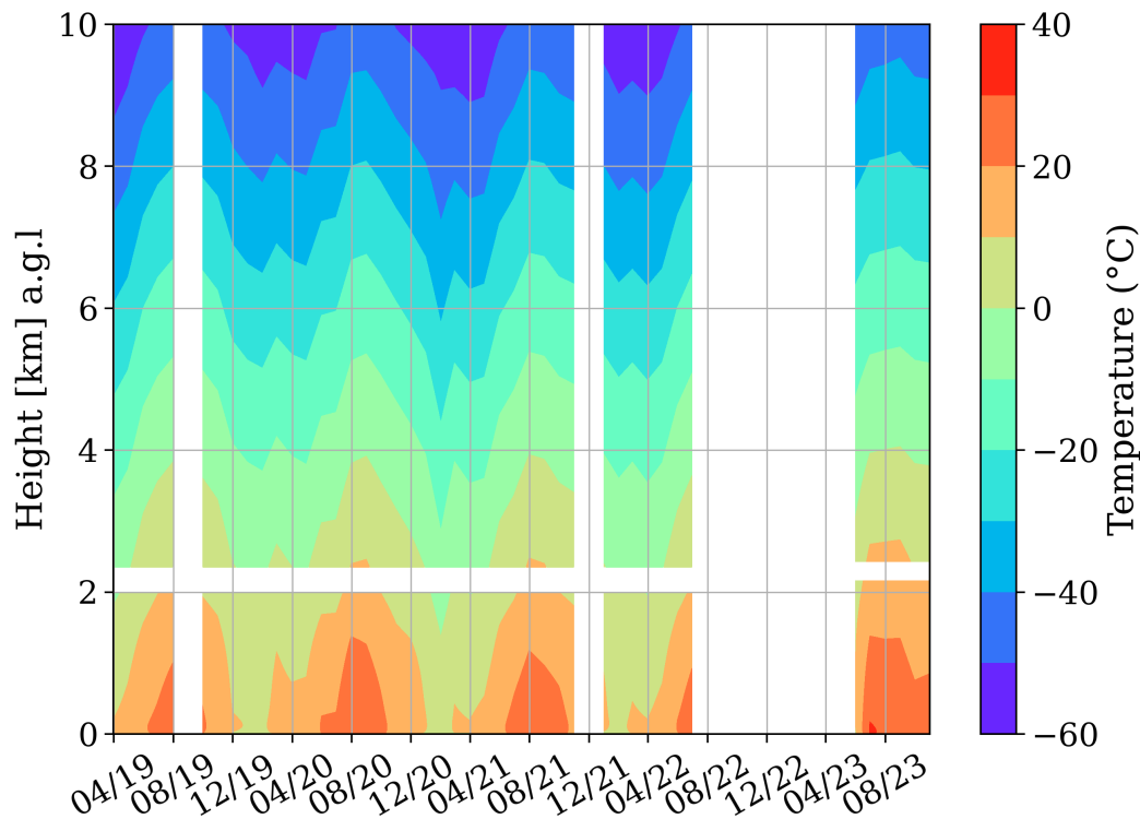
Figure 4. Monthly evolution of averange temperature and humidity profiles obtained with the microwave radiometer.
