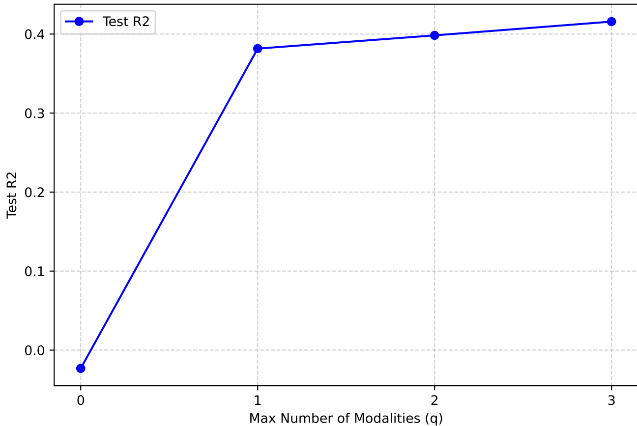
Model Selection Path
