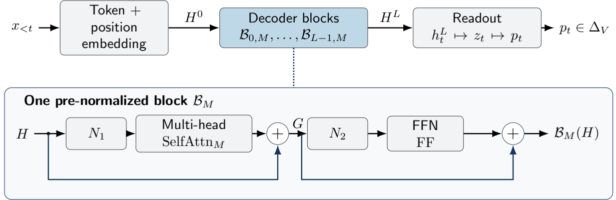
Figure 2: An archetypical decoder transformer as a composition of maps. A prefix x_{<t} is embedded as H^0 , transformed by L decoder blocks, and read out from the last row of H^L to produce logits z_t and the next-token distribution p_t . The inset expands one block: N_1, N_2 are positionwise normalization maps, \text{SelfAttn}_M exchanges information across positions allowed by mask M , and the feed-forward network (FFN) applies FF independently at each position. Blue paths carry the inputs to the two residual additions. All block inputs and outputs have shape T \times d . The labels abbreviate \mathcal{B}_{\ell,M} = \mathcal{B}_{\theta_\ell,M} and suppress the inset’s fixed component parameters. Different blocks may have different parameters; within a block, parameters are shared across positions and sequence lengths.
