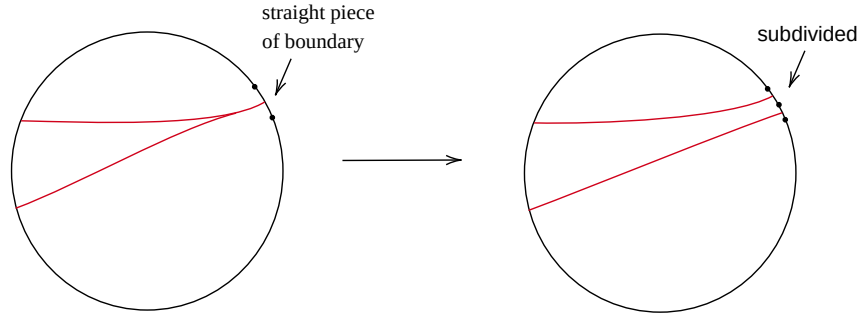
Figure 26: A 1-loop.
