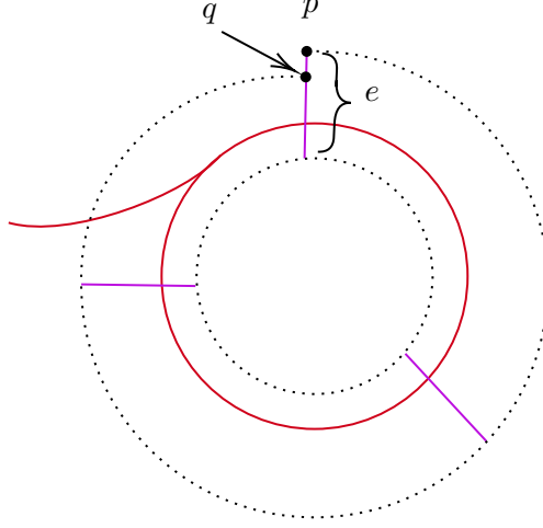
Figure 21: A 0-gon with a single switch. The edge e is embedded in M , but the points p and q are identified, which is impossible.
