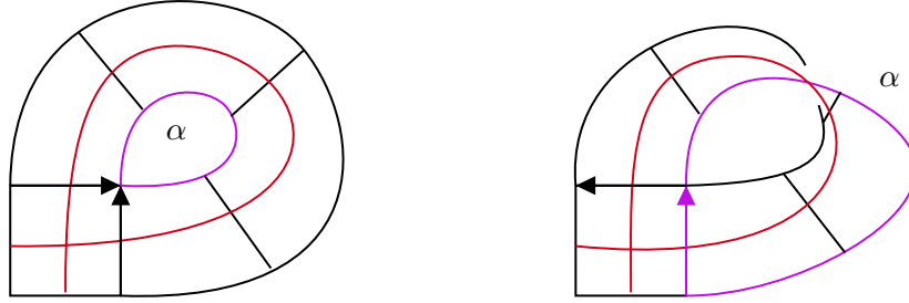
Figure 28: Two ways a regular leaf can self-intersect.
