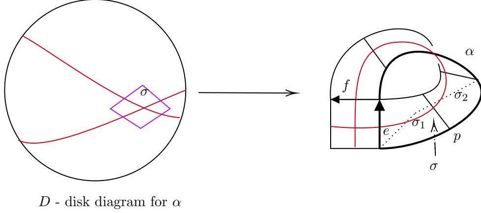
Figure 29: The corner of the disk diagram provides a new square at p .
