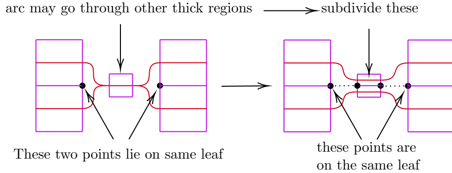
Figure 16: A middle splitting.
