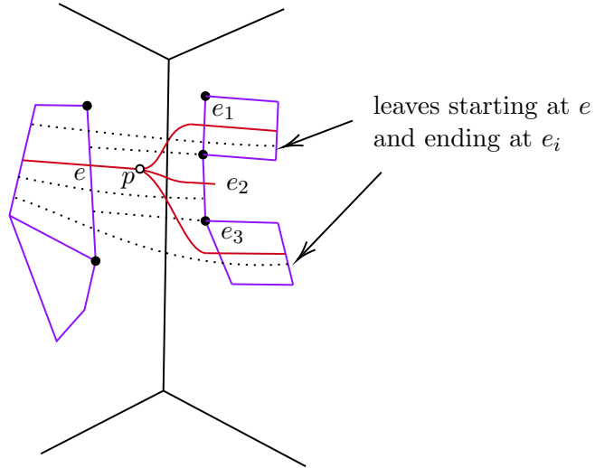
Figure 9: Building the train tracks. The track leaving the edge is given a switch point so that it can locally carry the leaves between the corresponding edges.
