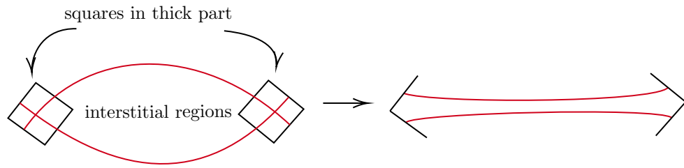
Figure 23: A bigon move removes two crossings.
