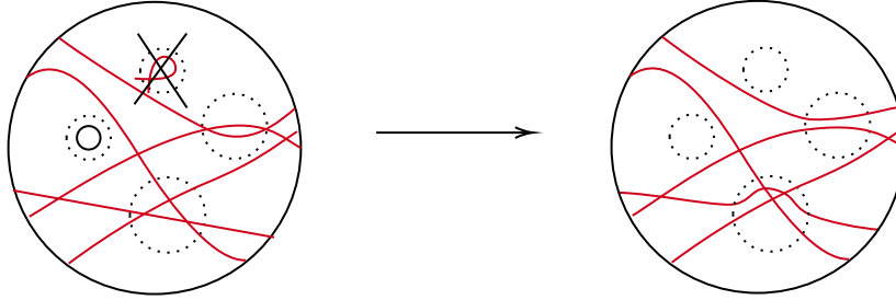
Figure 2: The elementary moves.
