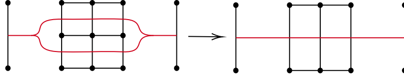
Figure 24: A bigon move eliminating two switches.
