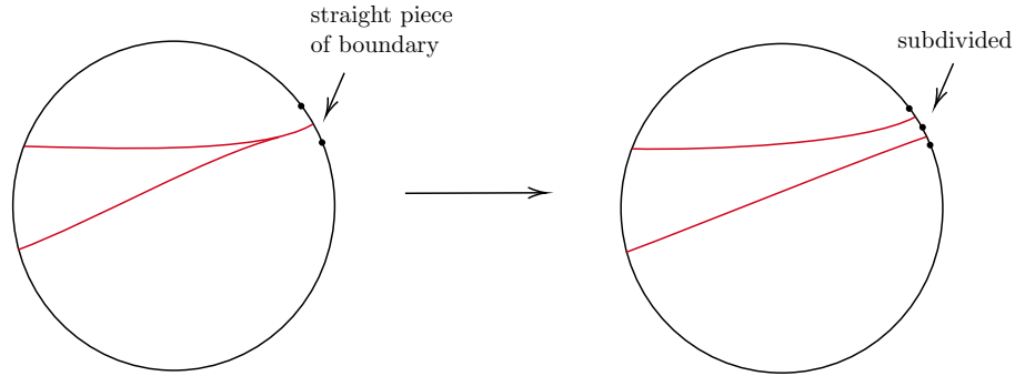
Figure 27: When the slide reaches the boundary.
