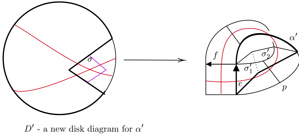
Figure 30: Replacing the band with a new band and a smaller disk diagram.
