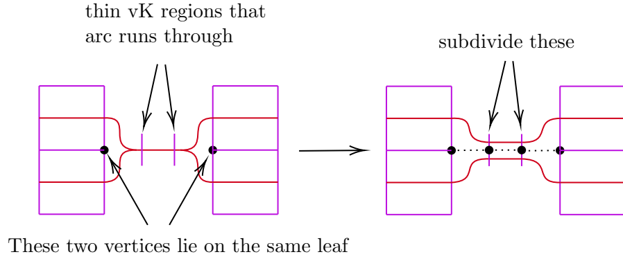
Figure 16: A central split.
