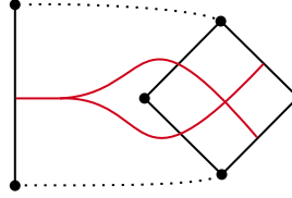
Figure 25: A bigon with a switch and a crossing means that the straight path on the left is identified with the not straight path on the right.
