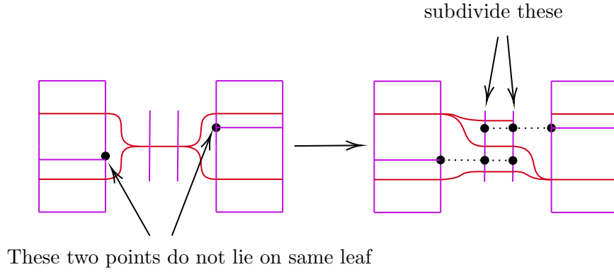
Figure 17: A right split.
