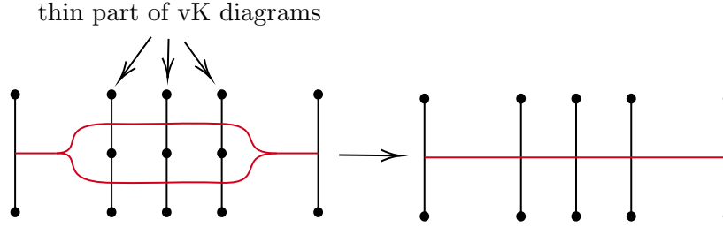
Figure 24: A bigon move eliminating two switches.
