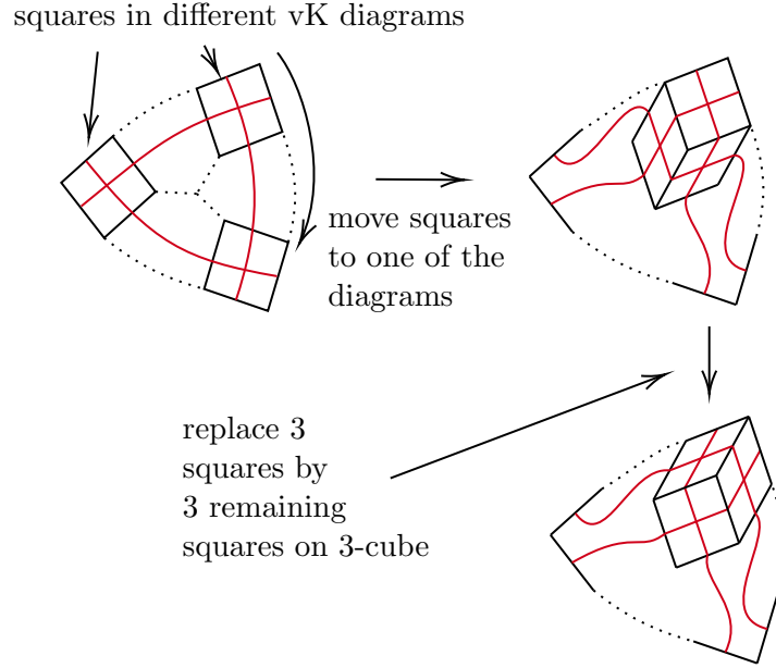
Figure 26: A triangle move.
