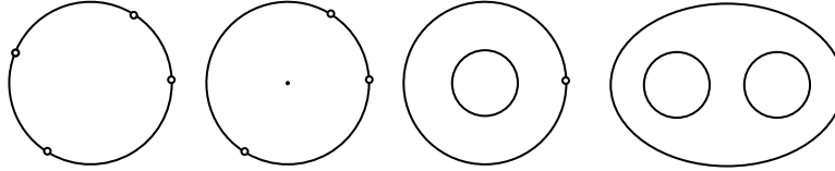
FIGURE 23. The topological possibilities for the components of S_0 .
