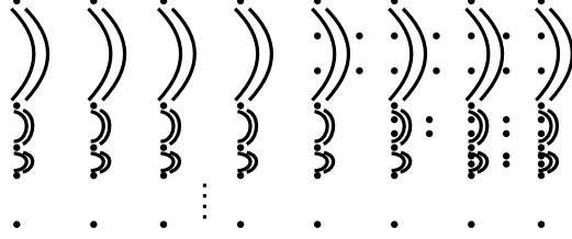
FIGURE 16. The modified surface in Example 7.9.
