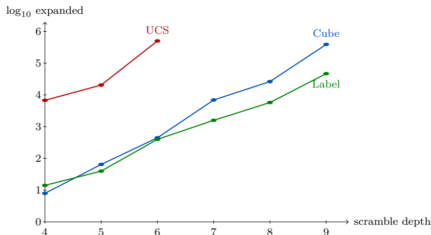
Figure 5: Expanded states by depth, log scale. UCS grows much faster and stops near depth six within memory. Both A* curves stay low, with the sticker heuristic below the piece one.
