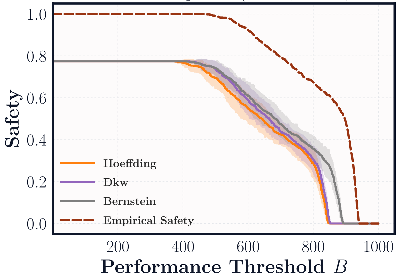
Bounds Comparison ( n = 100, m = 300 )
