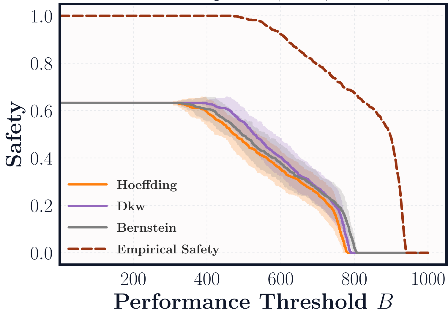
Bounds Comparison ( n = 50, m = 100 )
